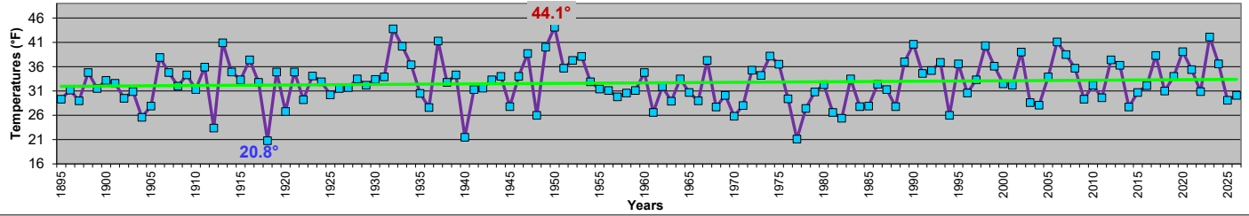
Maryland - February Mean Temperatures 1895-2026
