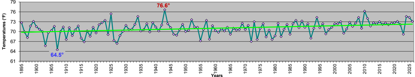
Maryland - June Mean Temperatures 1895-2026
