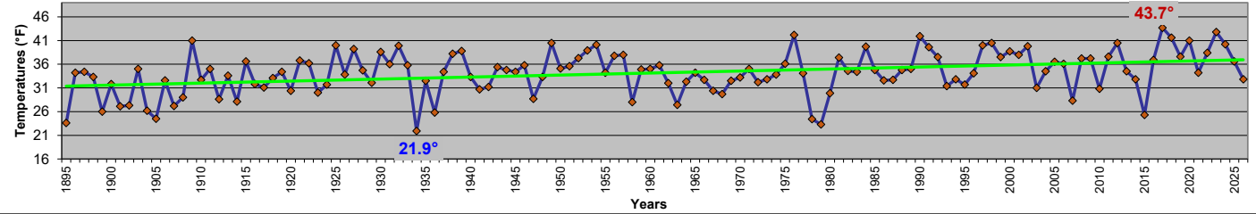
Maryland - March Mean Temperatures 1895-2026
