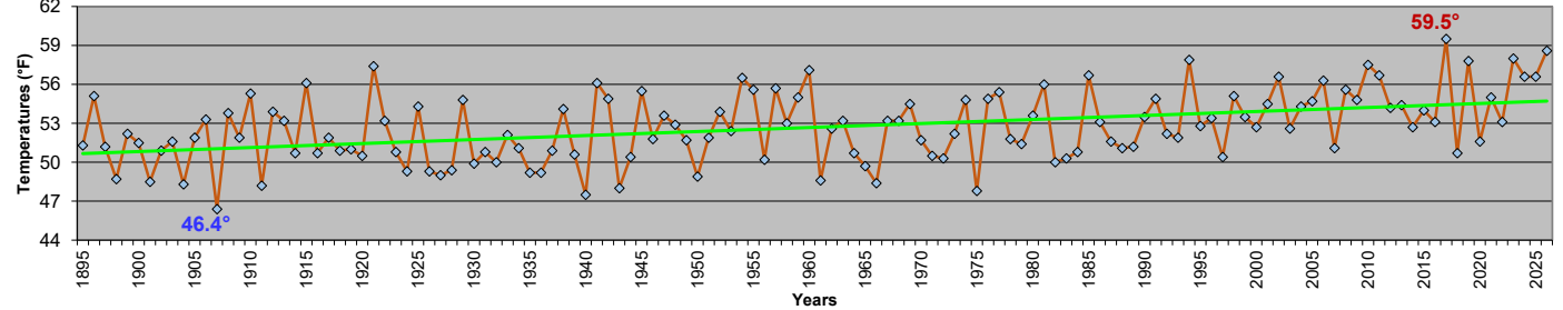
Maryland - May Mean Temperatures 1895-2026
