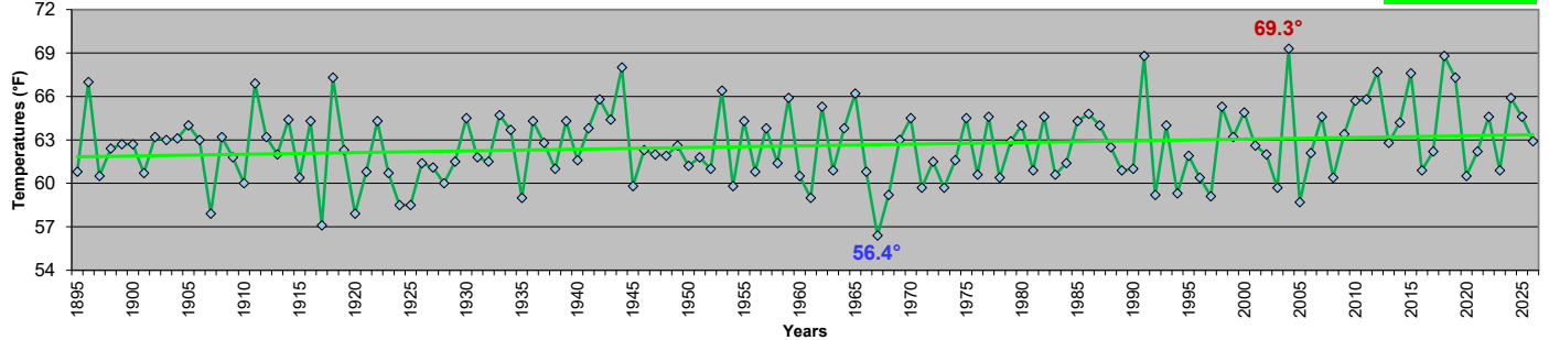
Maryland - June Mean Temperatures 1895-2026
