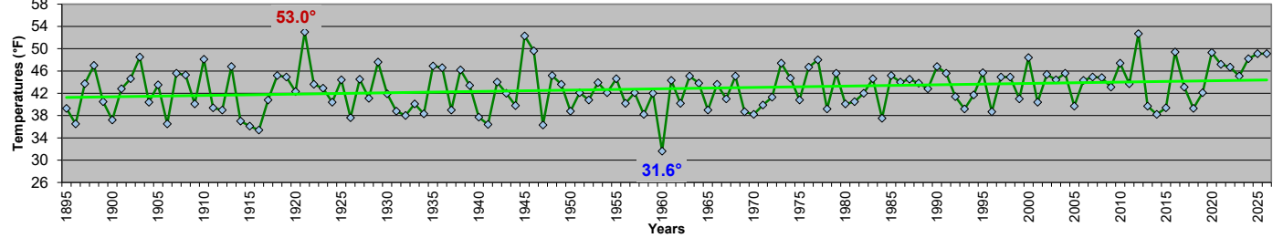
Maryland - April Mean Temperatures 1895-2026
