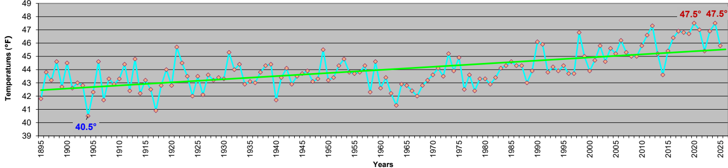
Maryland - Annual Average Minimum Temperatures 1895-2025
