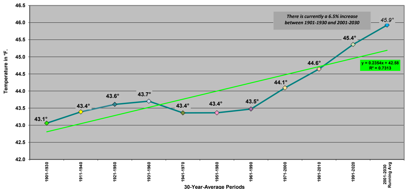
Maryland Statewide Annual Average Minimum Temperatures by 30-Year Averages, with associated Trendline
