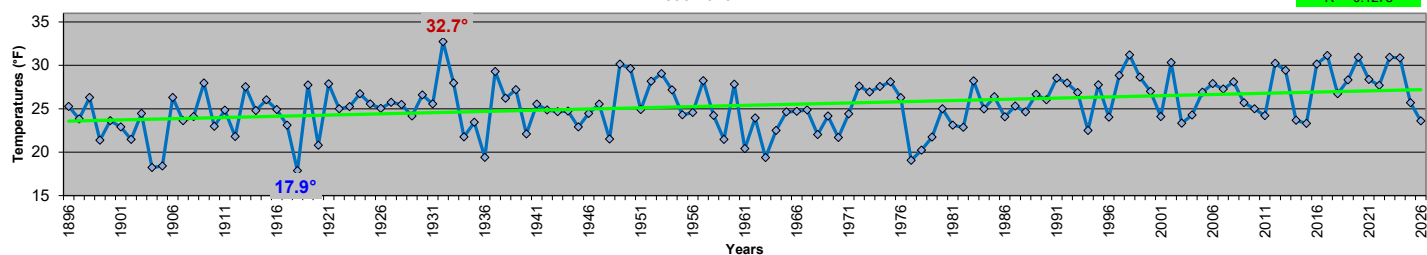
Maryland - Winter Average Minimum Temperatures (December-February) 1895-2026
