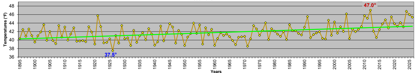
Maryland - Spring Average Minimum Temperatures (March-May) 1895-2026
