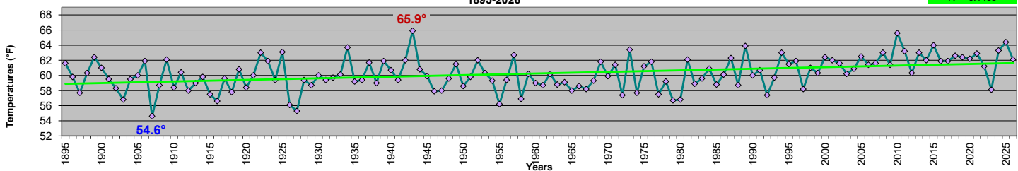
Maryland - June Average Minimum Temperatures 1895-2026
