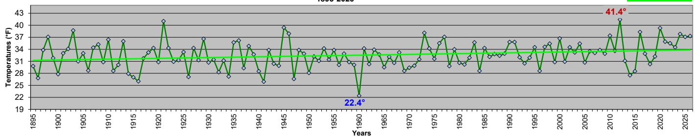
Maryland - April Average Minimum Temperatures 1895-2026
