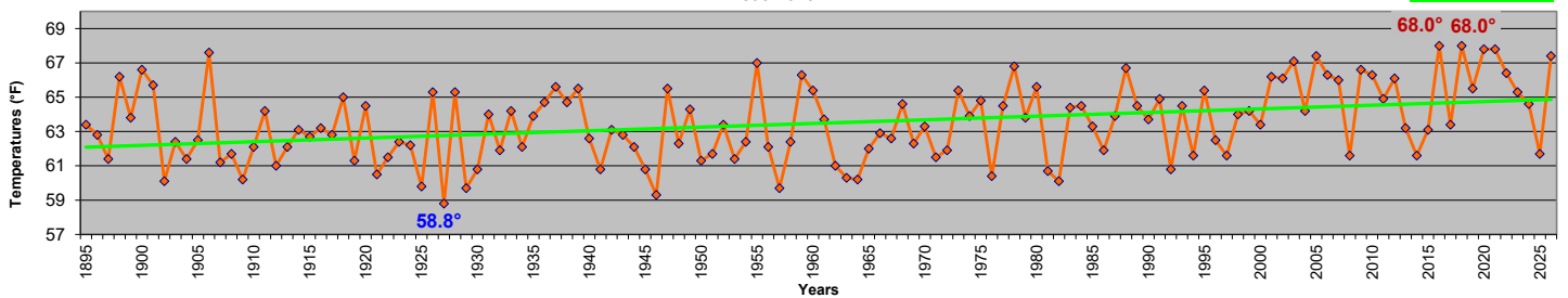
Maryland - September Average Minimum Temperatures 1895-2025
