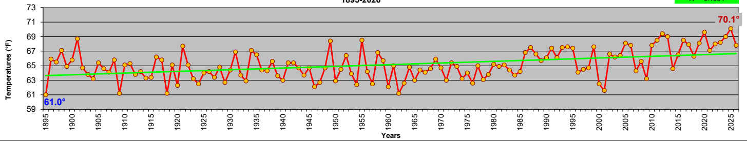
Maryland - August Average Minimum Temperatures 1895-2026
