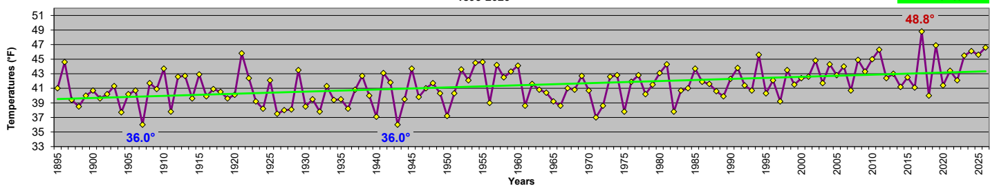
Maryland - May Average Minimum Temperatures 1895-2026
