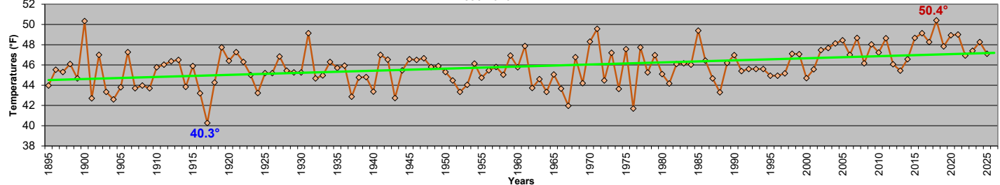
Maryland - Autumn Average Minimum Temperatures (September-November) 1895-2025
