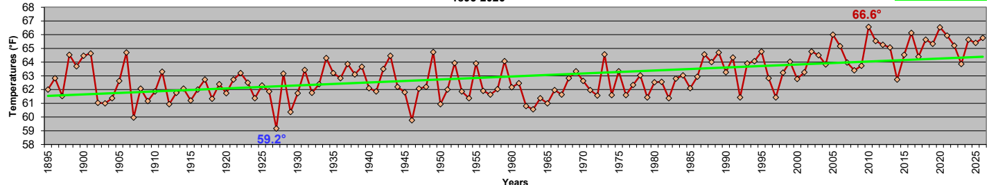
Maryland - Summer Average Minimum Temperatures (June-August) 1895-2026
