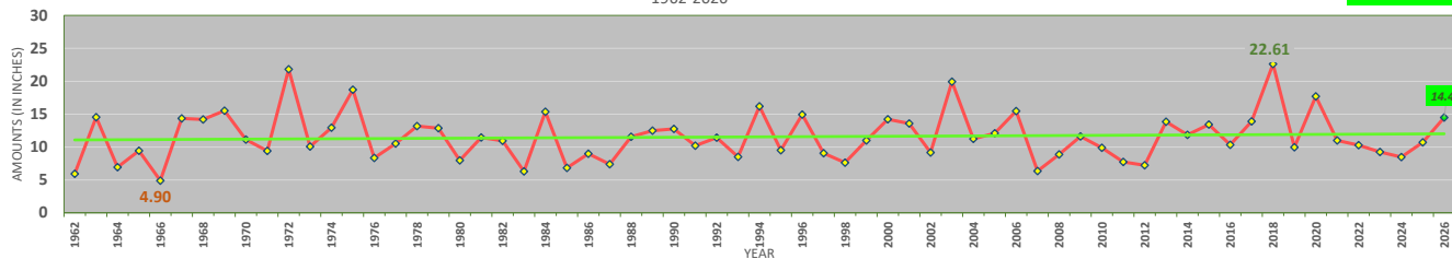
Washington-Dulles International Airport - Autumn Precipitation (September-November) (including Trendline and Extremes) 1962-2025
