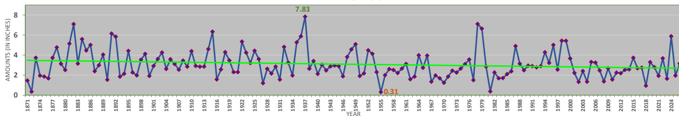
Washington, District of Columbia - February Precipitation (including Trendline and Extremes) 1871-2026
