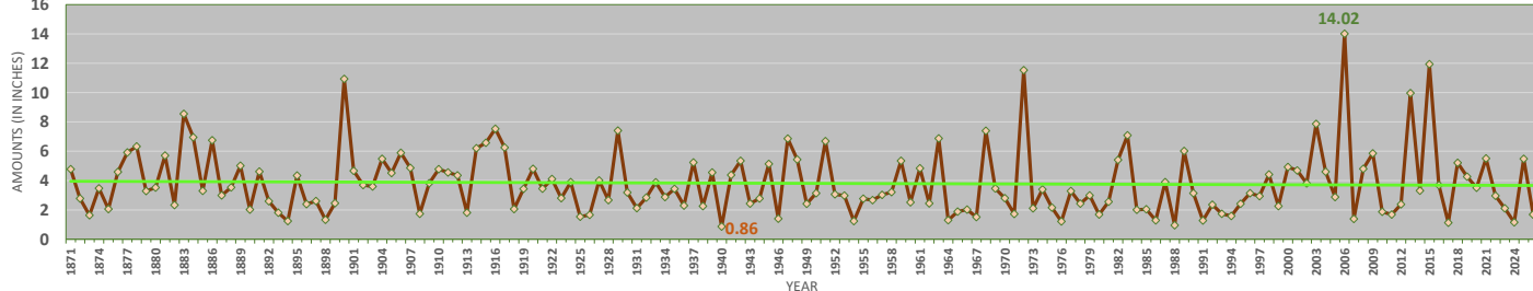
Washington, District of Columbia - June Precipitation (including Trendline and Extremes) 1871-2026
