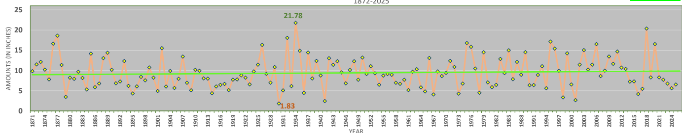
Washington, District of Columbia - Autumn Precipitation (September-November) (including Trendline and Extremes)
