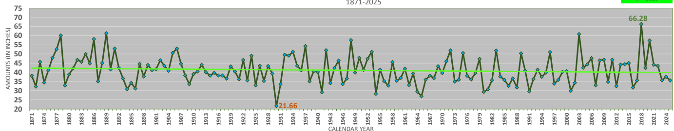
Washington, District of Columbia - Calendar-Year Precipitation (including Trendline and Extremes)
