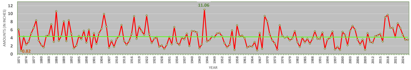
Washington, District of Columbia - August Precipitation (including Trendline and Extremes) 1871-2026
