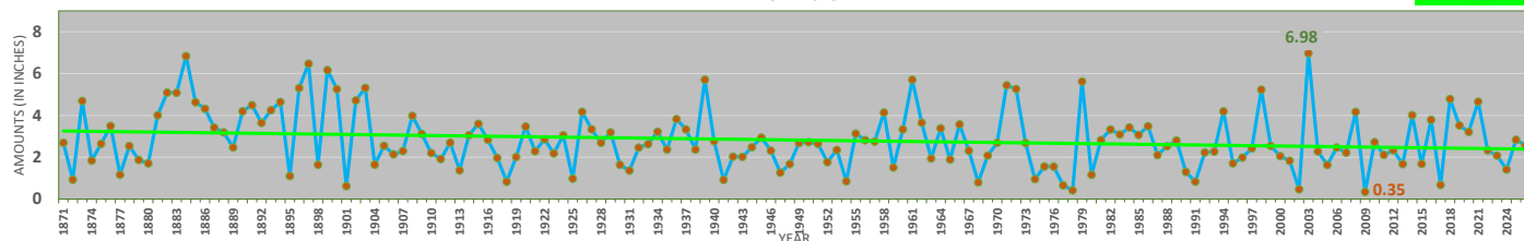
Washington, District of Columbia - March Precipitation (including Trendline and Extremes) 1871-2026
