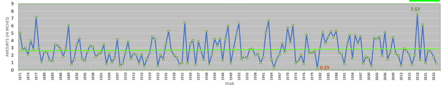
Washington, District of Columbia - December Precipitation (including Trendline and Extremes) 1871-2025
