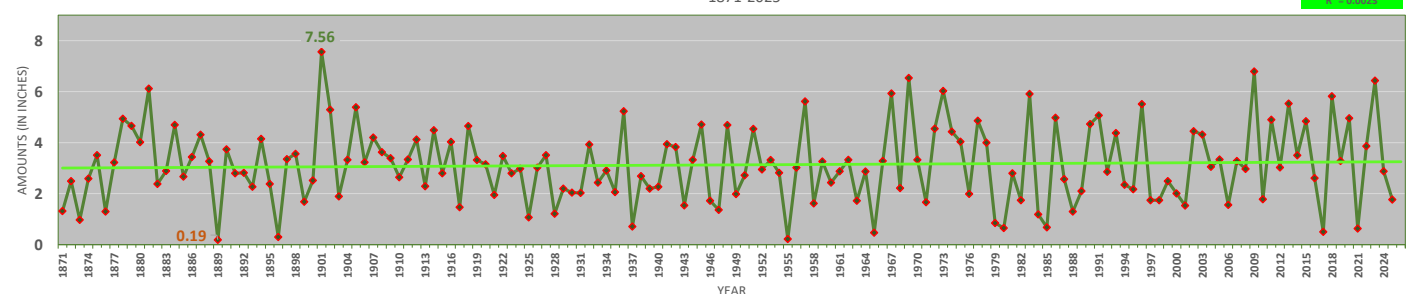
Washington, District of Columbia - December Precipitation (including Trendline and Extremes) 1871-2025
