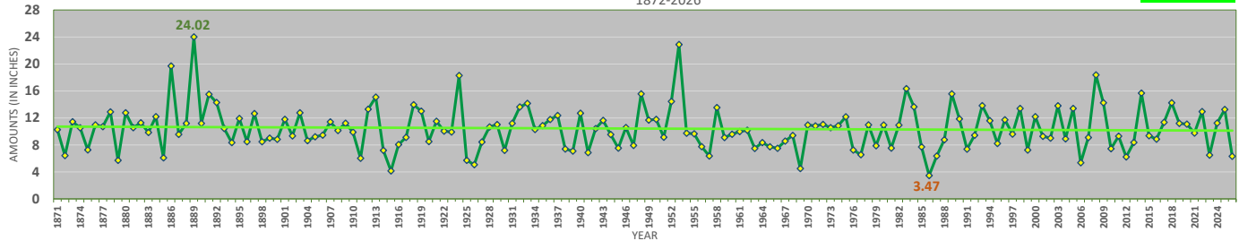
Washington, District of Columbia - Summer Precipitation (June-August) (including Trendline and Extremes)
