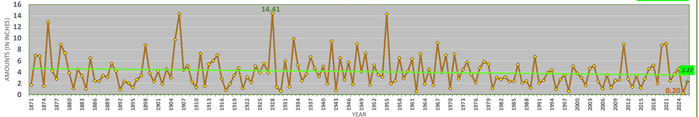
Washington, District of Columbia - September Precipitation (including Trendline and Extremes) 1871-2025
