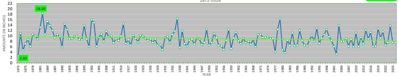
Washington, District of Columbia - Spring Precipitation (March-May) (including Trendline and Extremes)
