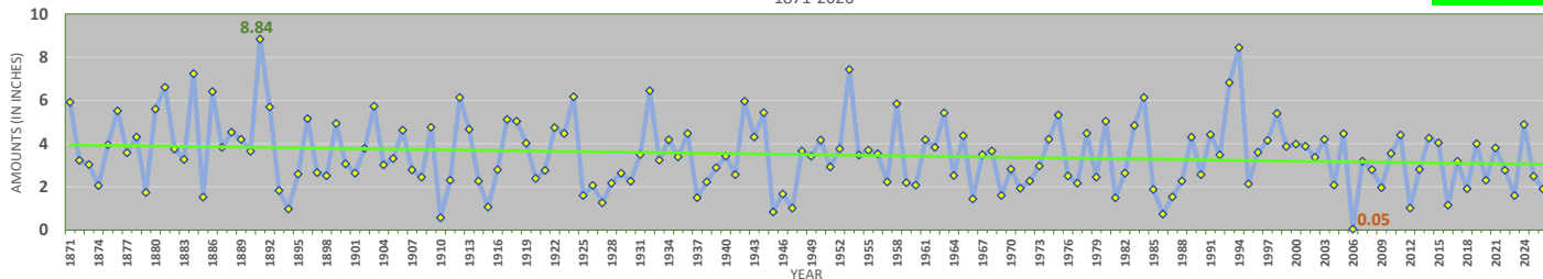
Washington, District of Columbia - April Precipitation (including Trendline and Extremes) 1871-2026
