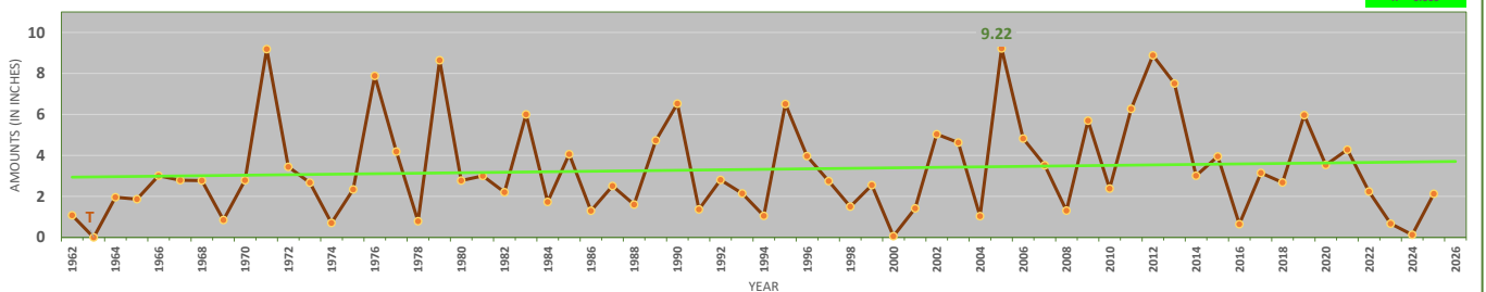
Washington-Dulles International Airport - November Precipitation (including Trendline and Extremes) 1962-2025
