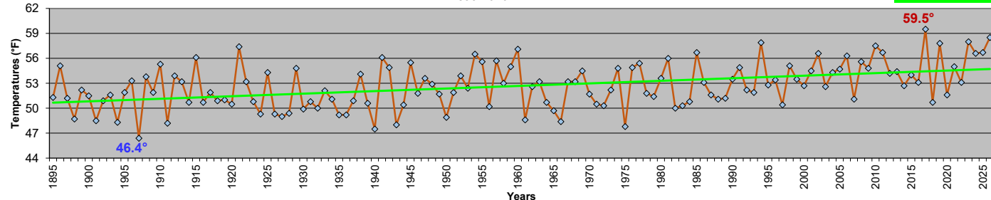
Maryland - May Mean Temperatures 1895-2026
