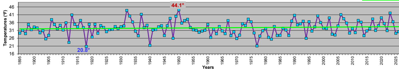
Maryland - February Mean Temperatures 1895-2026
