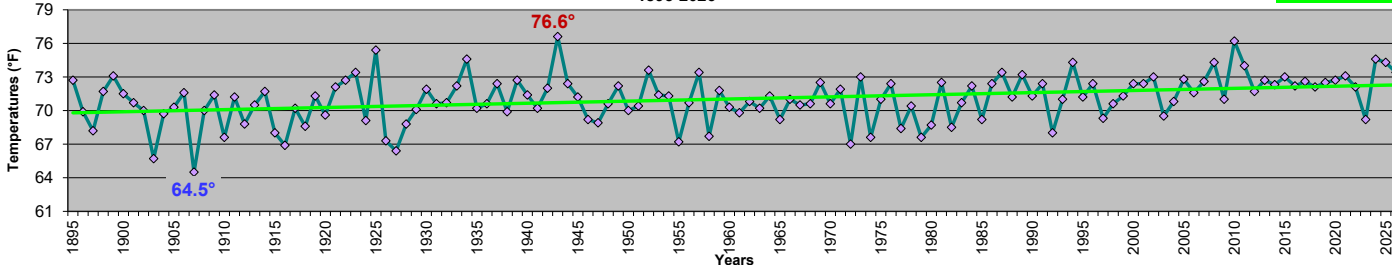
Maryland - June Mean Temperatures 1895-2026
