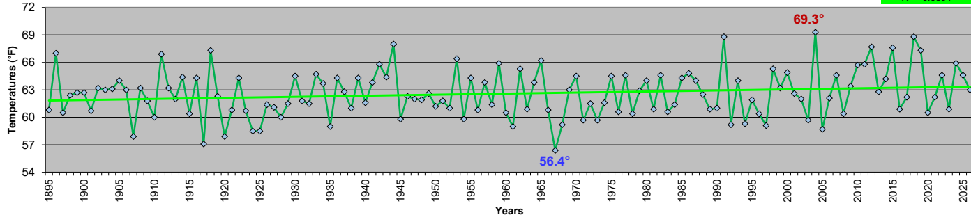
Maryland - June Mean Temperatures 1895-2026
