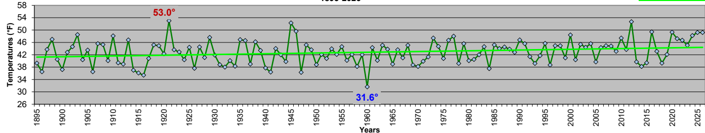
Maryland - April Mean Temperatures 1895-2026
