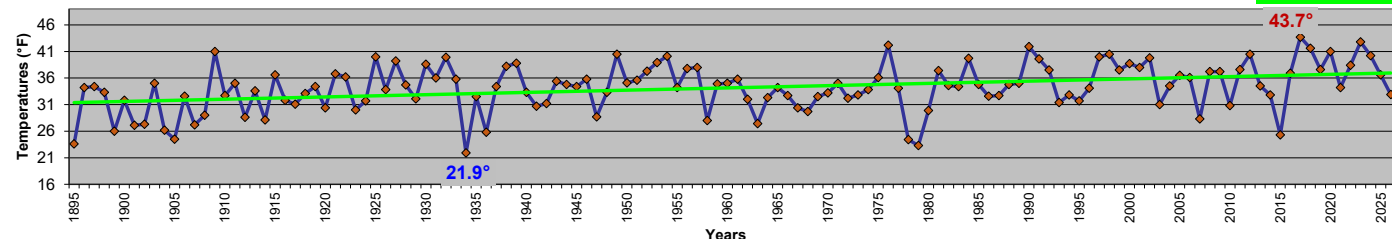
Maryland - March Mean Temperatures 1895-2026
