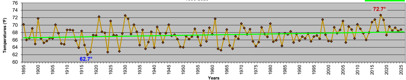
Maryland - September Mean Temperatures 1895-2025
