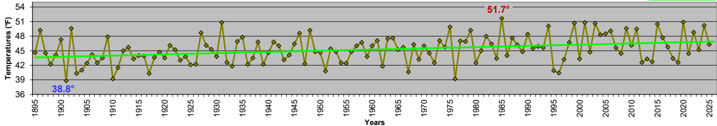
Maryland - December Mean Temperatures 1895-2025
