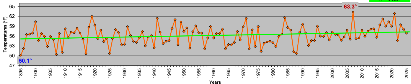
Maryland - November Mean Temperatures 1895-2025
