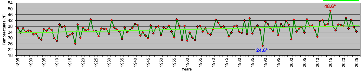
Maryland - December Mean Temperatures 1895-2025
