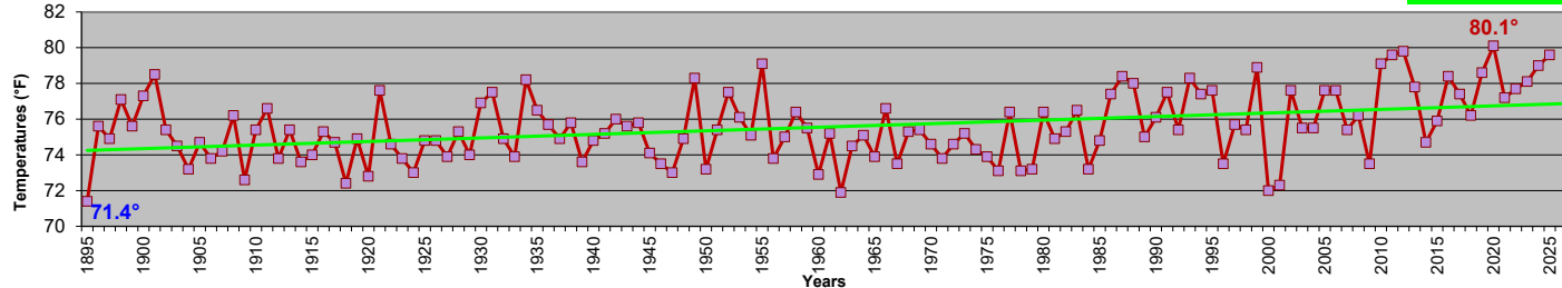
Maryland - July Mean Temperatures 1895-2025
