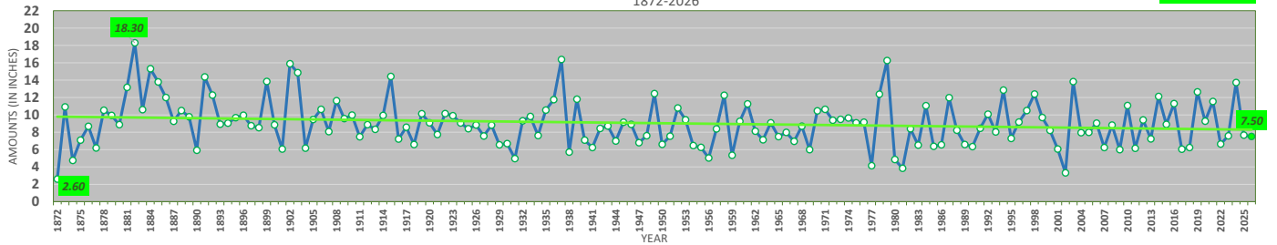
Washington, District of Columbia - Spring Precipitation (March-May) (including Trendline and Extremes) 1872-2026
