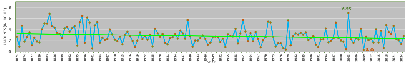
Washington, District of Columbia - March Precipitation (including Trendline and Extremes)
