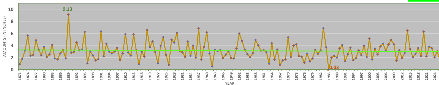
Washington, District of Columbia - May Precipitation (including Trendline and Extremes)
