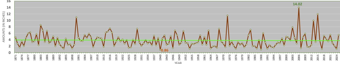
Washington, District of Columbia - June Precipitation (including Trendline and Extremes)
