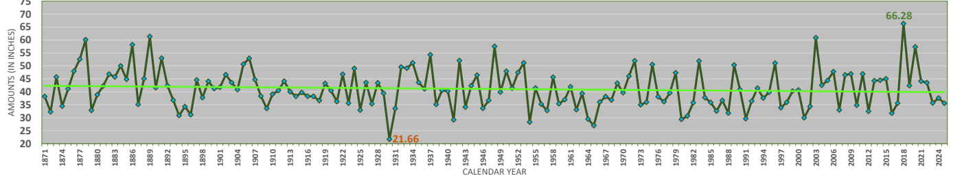
Washington, District of Columbia - Calendar-Year Precipitation (including Trendline and Extremes) 1871-2025
