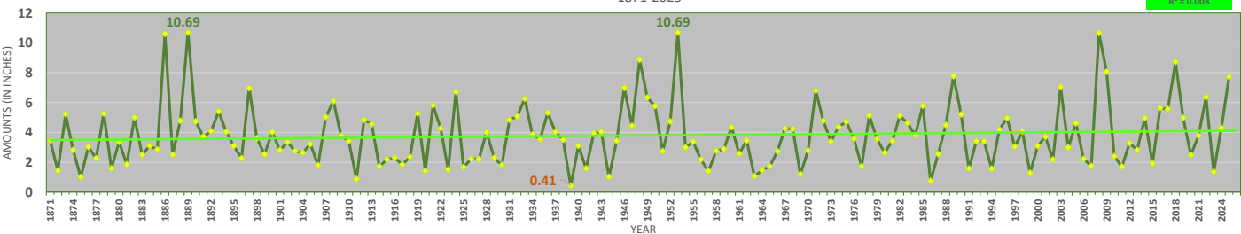
Washington, District of Columbia - June Precipitation (including Trendline and Extremes) 1871-2025
